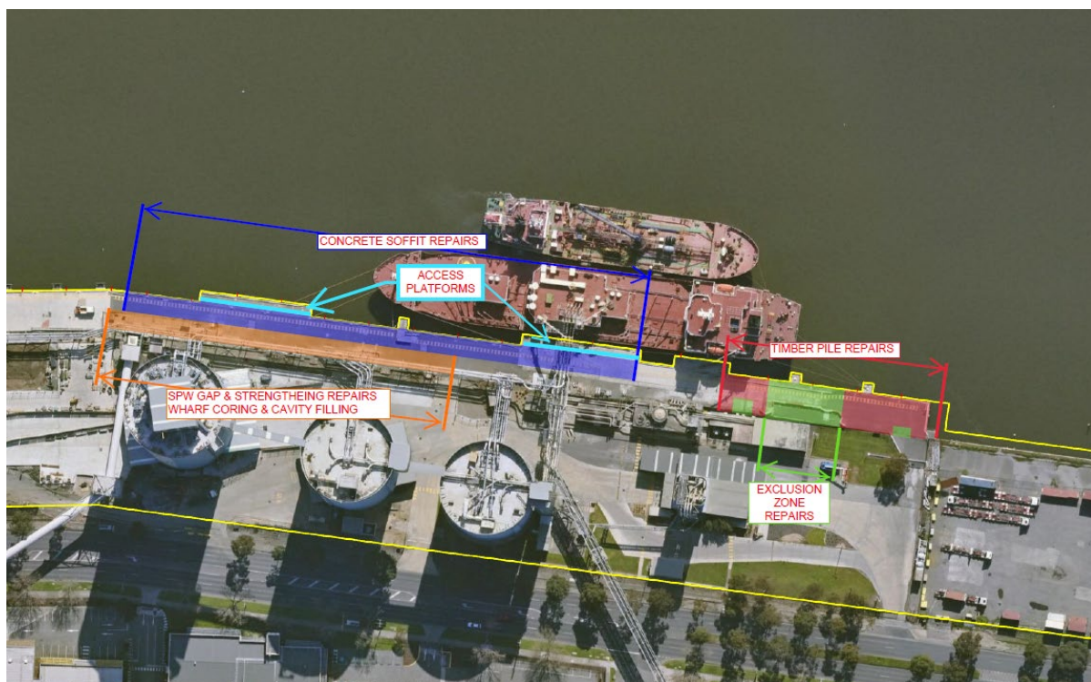
SOUTH WHARF 26 - WORKS PLAN
