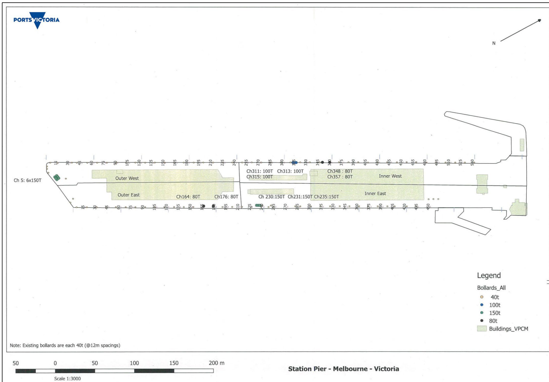
Diagram 3(g) Station Pier general arrangement plan
