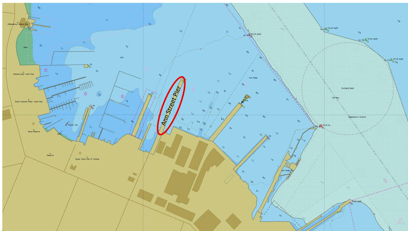
ANN STREET PIER - SITE PLAN
