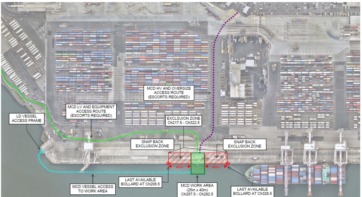
SWANSON DOCK BERTH 1 WEST - SITE PLAN AND SNAPBACK ZONE
